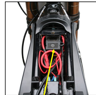
Main fuse
